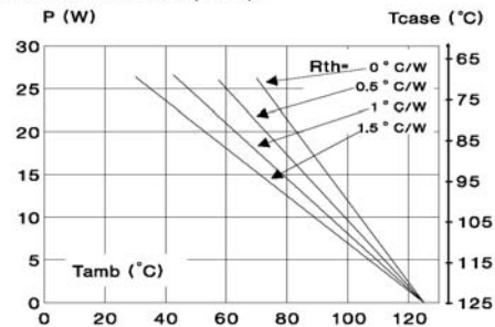
Fig. 2: Correlation between maximum RMS power dissipation and maximum allowable temperatures ( T_{\text{amb}} and T_{\text{case}} ) for different thermal resistances heatsink + contact (BTA).
