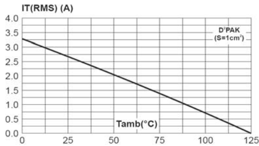
Fig. 2-2: D 2 PAK RMS on-state current versus ambient temperature (printed circuit board FR4, copper thickness: 35 μm), full cycle.
