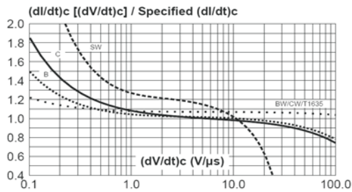
Fig. 8: Relative variation of critical rate of decrease of main current versus (dI/dt)_c (typical values).
